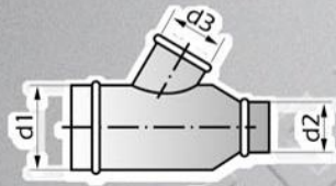
ÇATAL REDÜKSİYON SADDLE PIECE WITH REDUCER
