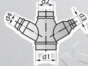
ÇATAL REDÜKSİYON COLLAR PIECE REDUCER
