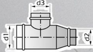
TE REDÜKSİYON 90° T-PIECE 90° WITH REDUCER
